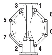
Torque Sequence
