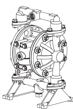
PD05P-ASS-XXX 1/2" POMPE A DIAPHRAGME ACIER INOXYDABLE
