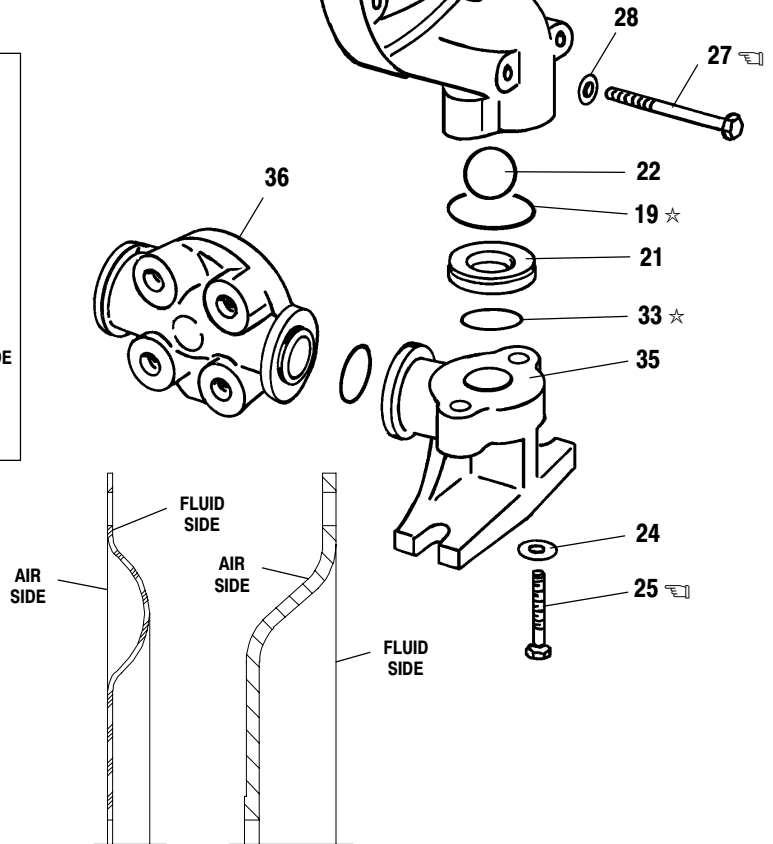
CROSS SECTION VIEW OF DIAPHRAGMS
